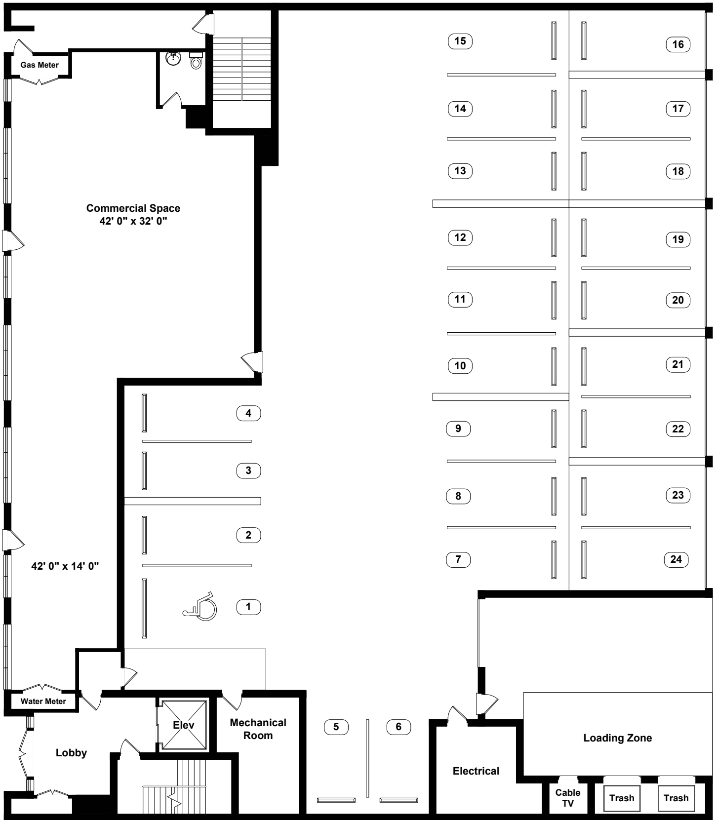
First Floor
